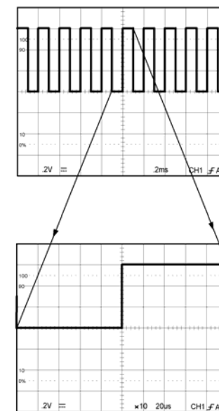
Figure 5-8 Magnified Waveform
